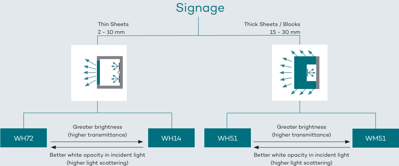
Fig. 3: Decision tree
