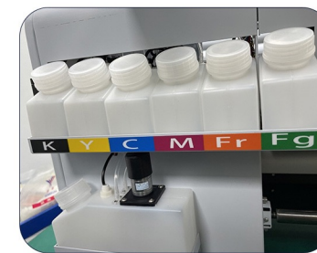
| Ink tank
