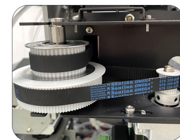
| Synchronous pulley
